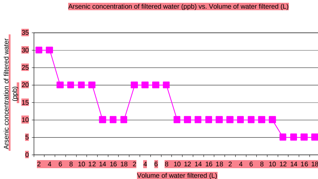
Figure 9: ABF 1 Arsenic concentration of filtered water (ppb) vs. Volume of Water filtered (L)
